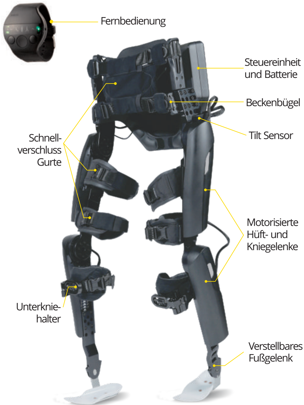
ReWalk 6.0 Exoskelett
